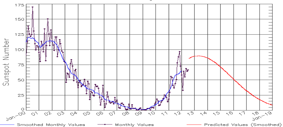
ISES Solar Cycle Sunspot Number Progression Observed data through Jul 2012
