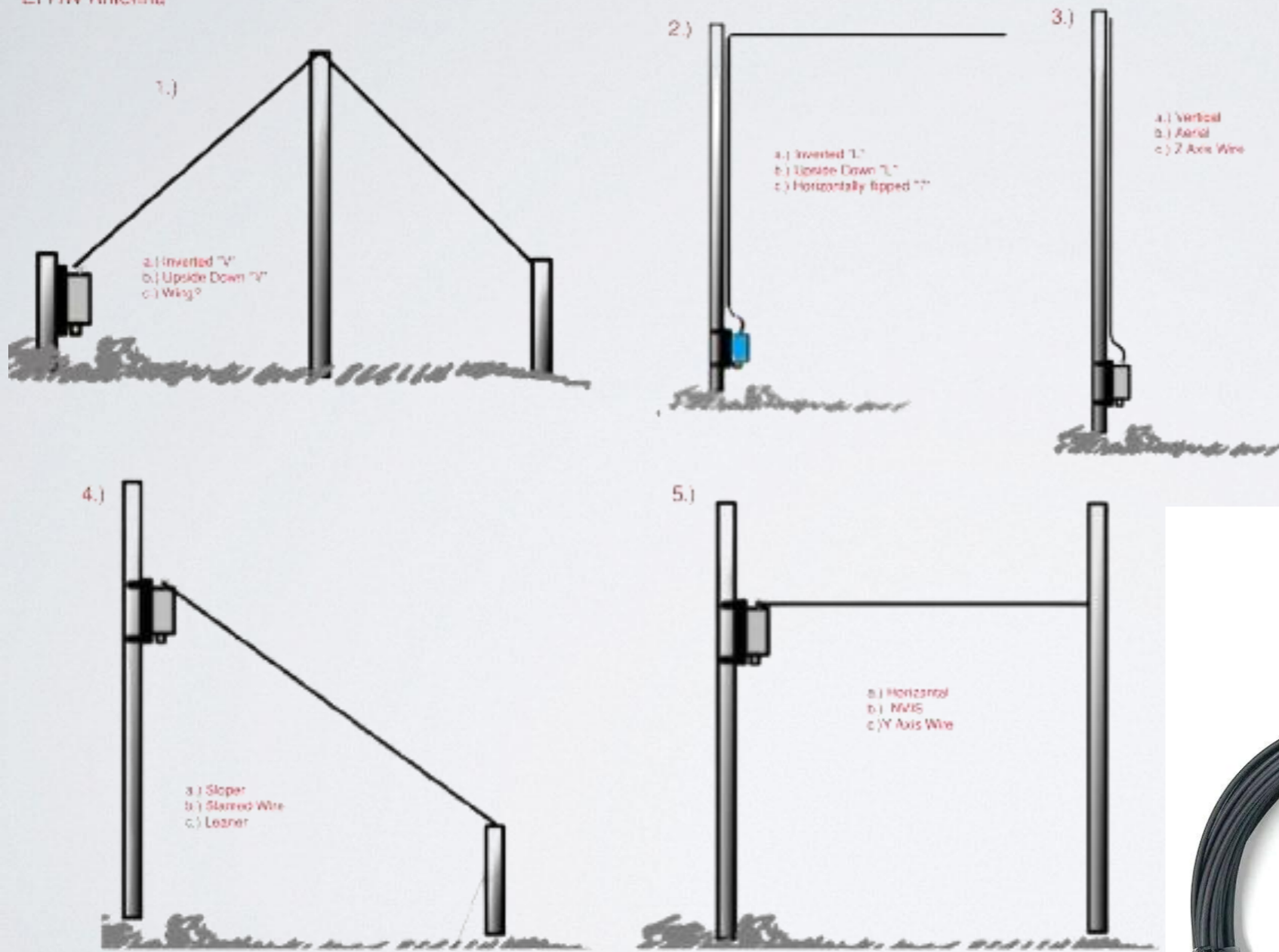
EFHW Antenna
